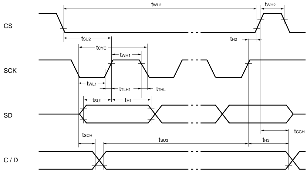
Fig. 2 Interface timing
