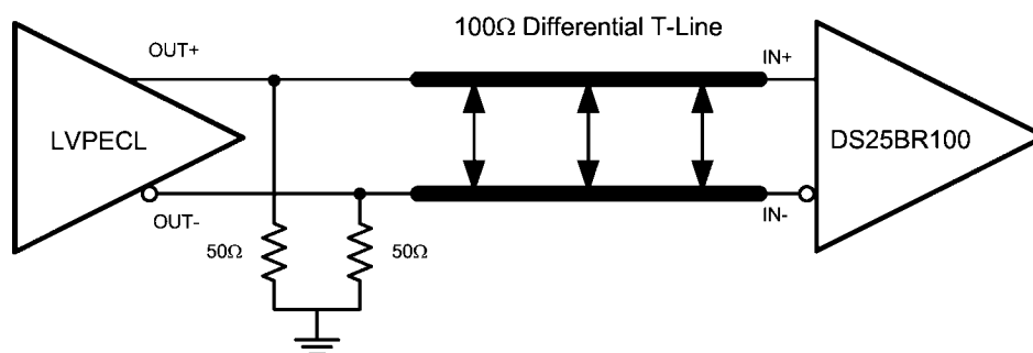
Typical LVPECL Driver DC-Coupled Interface to DS25BR100 Input
