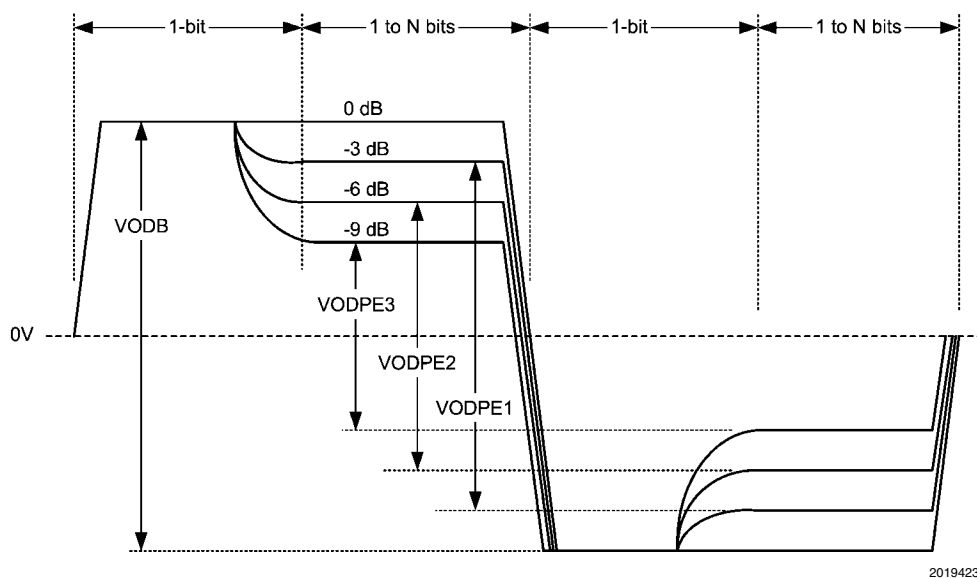
FIGURE 1. Driver De-Emphasis Differential Waveform (showing all 4 de-emphasis steps)
