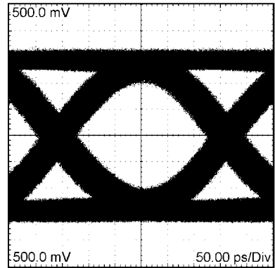
30003765 A 3.125 Gbps NRZ PRBS-23 with High PE After 30" Differential FR-4 Stripline H: 50 ps / DIV, V: 100 mV / DIV
