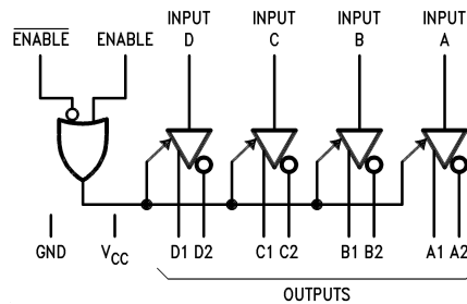
FIGURE 1. Logic Symbol
