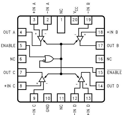
20-Lead Ceramic Leadless Chip Carrier See NS Package Number E20A
