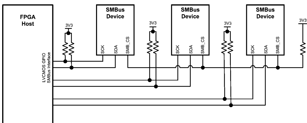
FIGURE 10. SMBus Configuration 3
