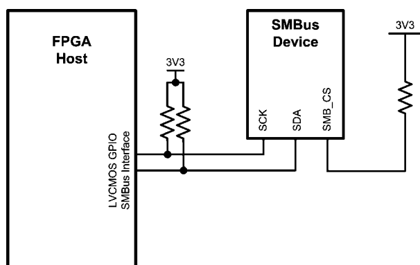
FIGURE 8. SMBus Configuration 1
