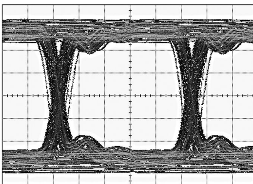
Figure 8. Equalized Signal (10m 24 AWG Twin-AX Cable, 3.2 Gbps, PRBS 7, 0x07 Setting)
