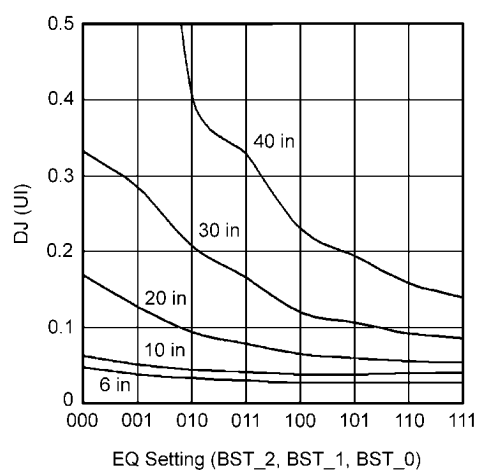
Figure 10. DJ vs. EQ Setting (3.2 Gbps)
