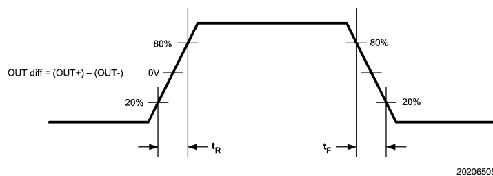
FIGURE 2. CML Output Transition Times
