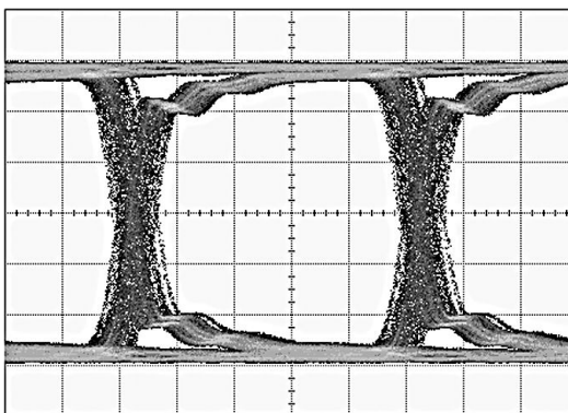
Figure 6. Equalized Signal (40 in FR4, 2.5 Gbps, PRBS 7, 0x07 Setting)
