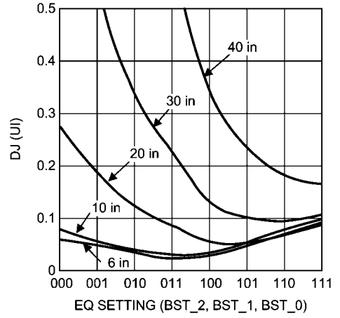
Figure 12. DJ vs. EQ Setting (6.4 Gbps)
