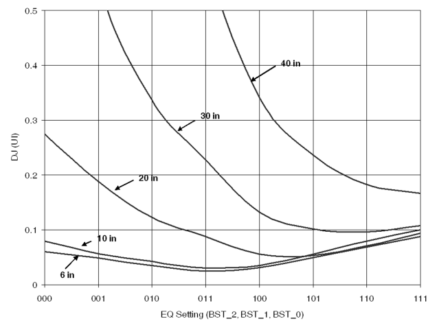
Figure 16. DJ vs EQ Setting (6.4 Gbps)
