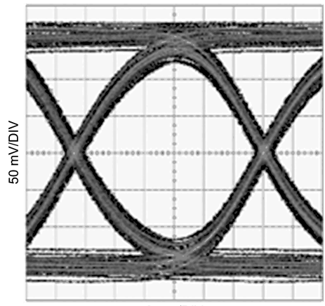
FIGURE 9. Equalized Signal (20in FR4, 6.25Gbps, PRBS7)
