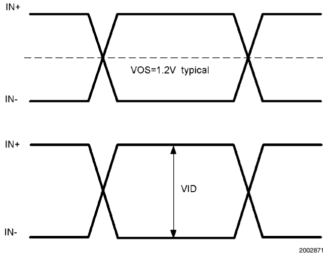
FIGURE 5. LVDS Signals
