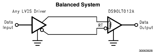
FIGURE 3. Point-to-Point Application (DS90LT012AQ)
