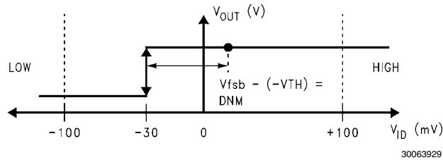
FIGURE 4. VTC of the DS90LT012AQ LVDS Receiver
