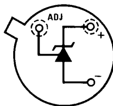
20139720 Bottom View See NS Package Number H03H
