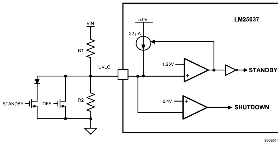
FIGURE 15. Remote Standby and Disable Control
