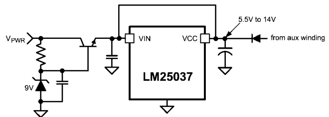
FIGURE 11. Start-up Regulator for V_{PWR} > 75\text{V}
