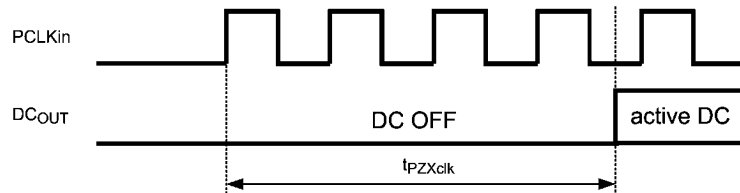
FIGURE 4. Stop Pixel Clock (PCLK) Power Up
