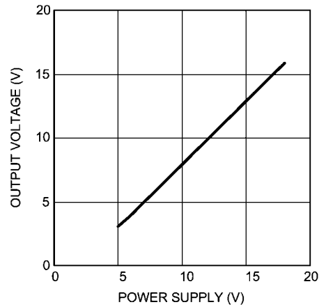
Output Voltage vs Supply Voltage A_V = 1V_{RMS}, R_L = 600\Omega
