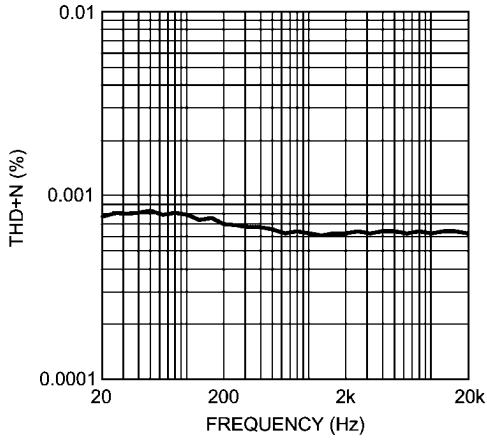
THD vs Frequency A_V = 3V_{RMS}, R_L = 100\Omega, SOIC
