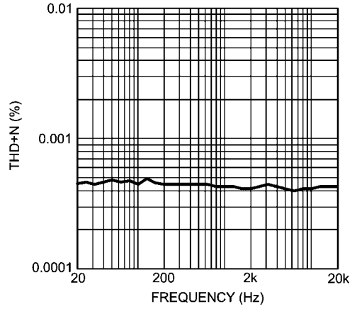
THD vs Frequency A_V = 3V_{RMS}, R_L = 600\Omega, SOIC
