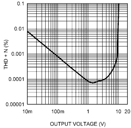
THD+N vs Output Voltage V_S = \pm 15V, R_L = 10k\Omega, f = 1kHz 30kHz BW
