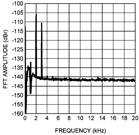
FFT of 1kHz Sinewave, 0dB Input Magnitude V_{OUT} = 3V_{RMS} , R_L = 1k\Omega , V_S = \pm 22V , A_V = 1
