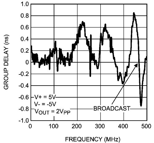
Group Delay
