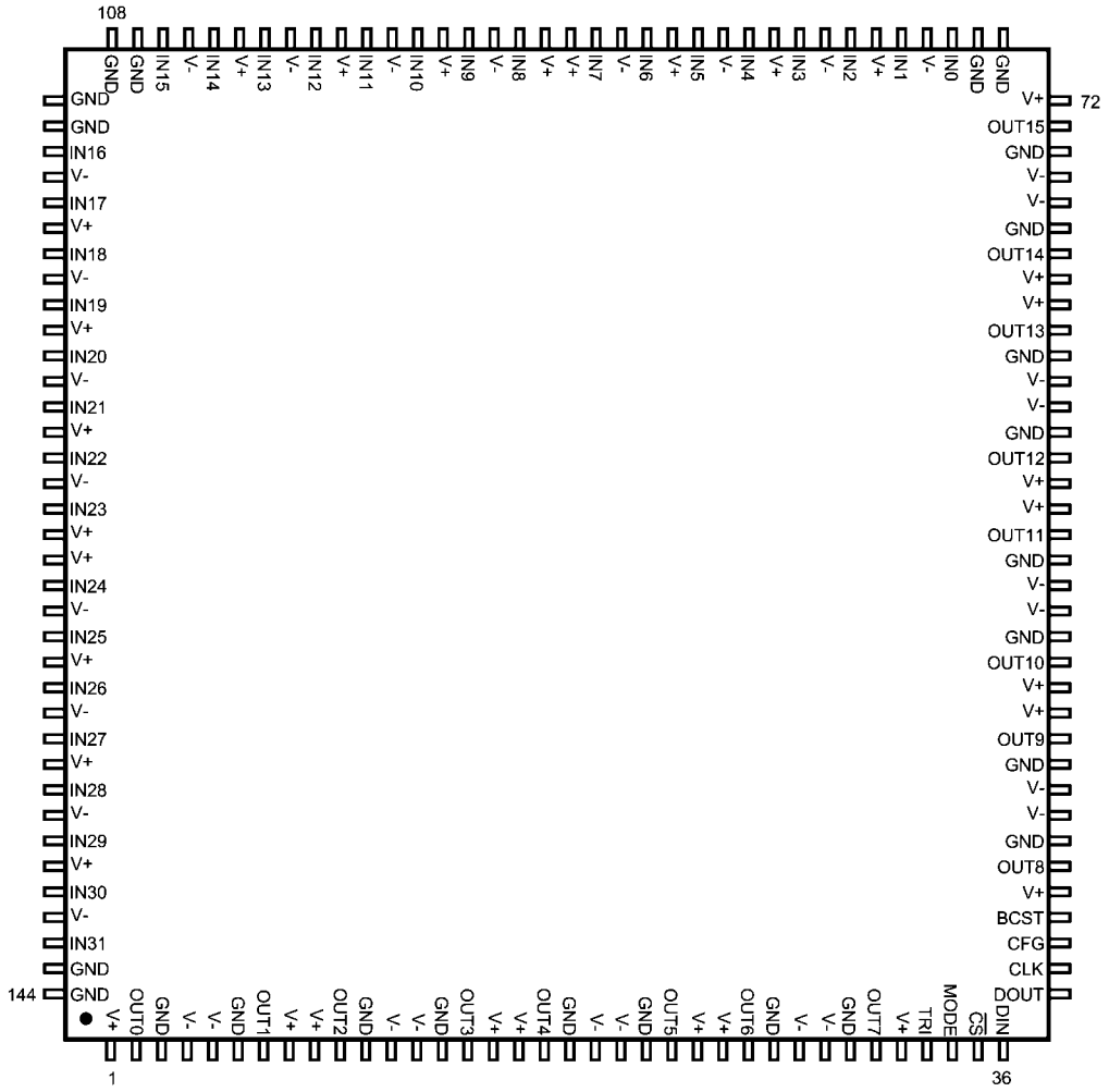
144-Pin LQFP
