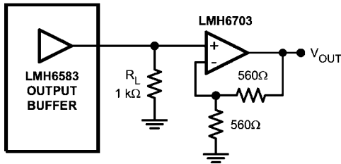
FIGURE 4. Buffered Output
