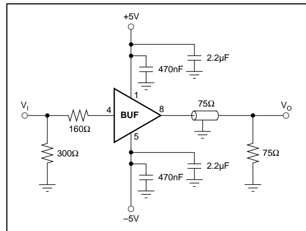
FIGURE 3. Impedance Converter.
