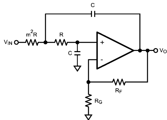
FIGURE 4. Sallen-Key Filter
