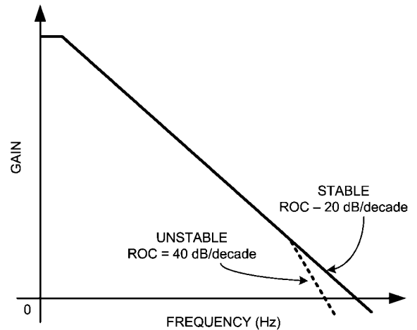
FIGURE 1. Gain vs. Frequency for an Op Amp
