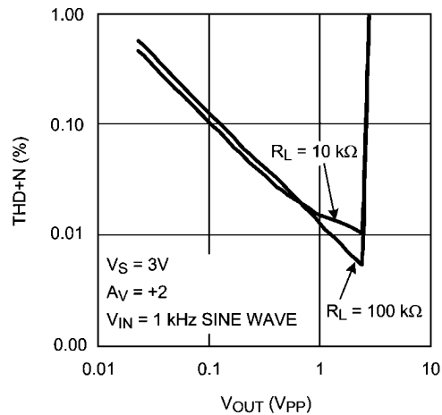
THD+N vs. Amplitude @ 3V
