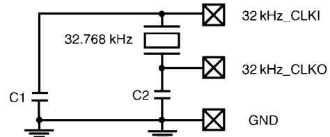
FIGURE 8. 32.768 kHz Oscillator
