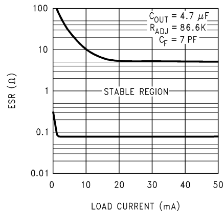
4.7 \mu\text{F} ESR Curves
