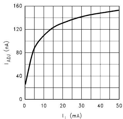
ADJ Pin Bias Current vs. Load Current
