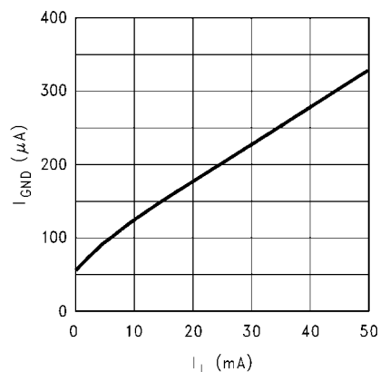
Ground Pin Current vs. Load Current
