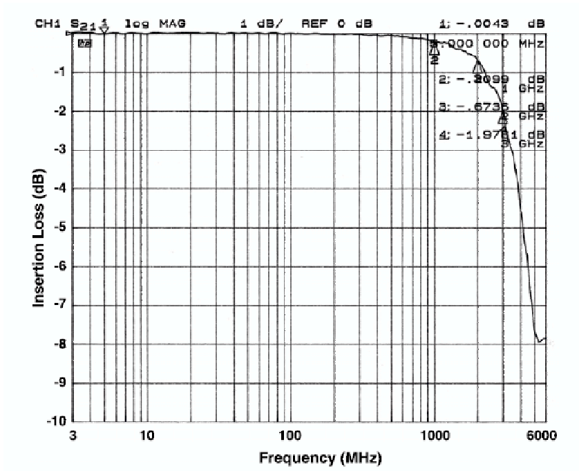
Figure 2. Insertion Loss vs. Frequency (TMDS_D1- to GND)
