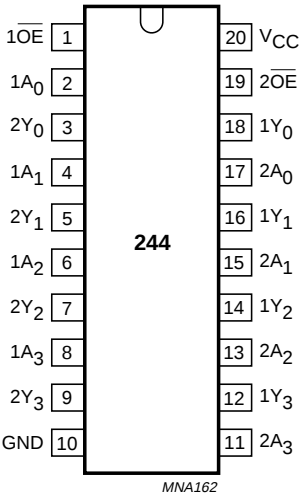
Fig.1 Pin configuration.
