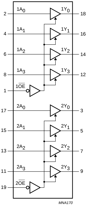
Fig.3 Logic diagram.
