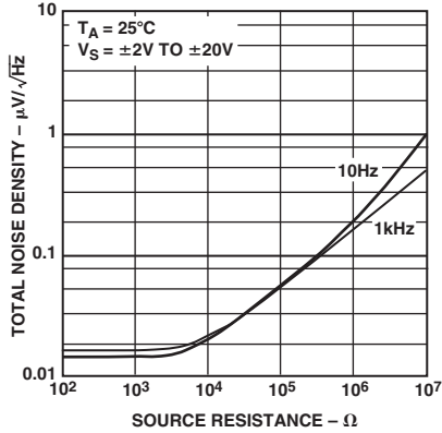
TPC 11. Total Noise Density vs. Source Resistance
