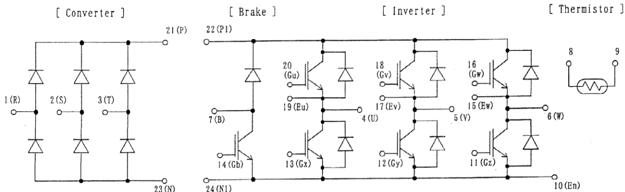
2. Equivalent circuit
