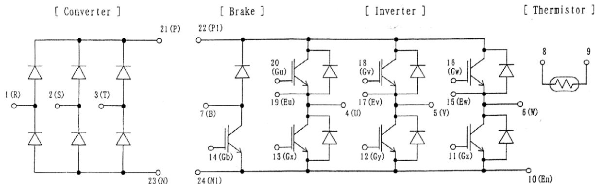
2. Equivalent circuit
