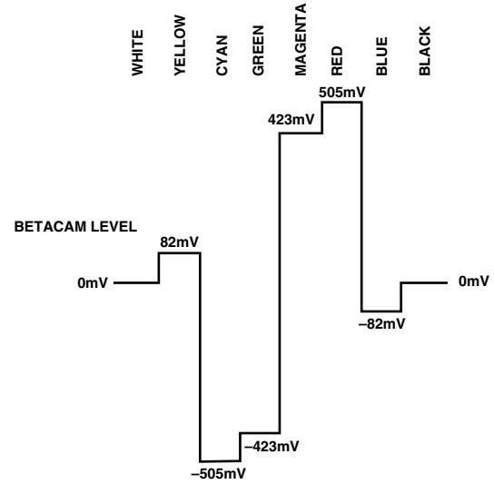
Figure 124. NTSC 100% Color Bars No Pedestal V Levels
