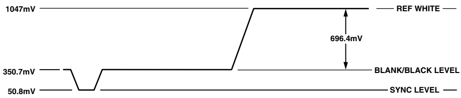
Figure 116. PAL Luma Video Levels
