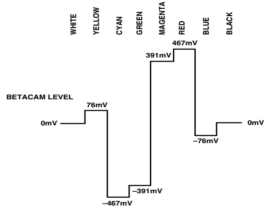
Figure 125. NTSC 100% Color Bars with Pedestal V Levels
