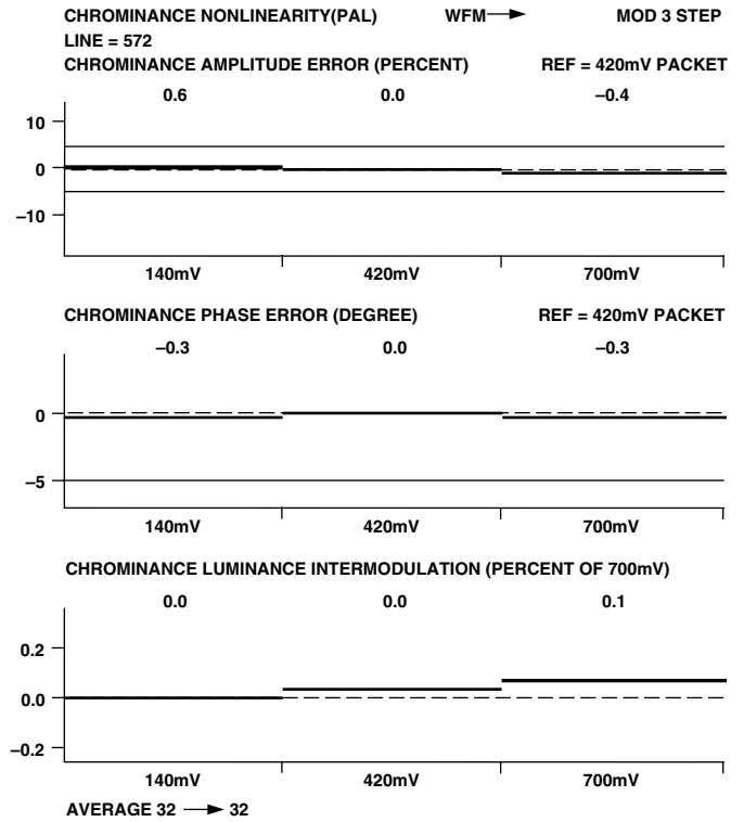
Figure 141. PAL Chrominance Nonlinearity
