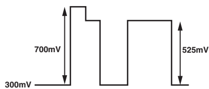
Figure 95. PS RGB Output Levels
