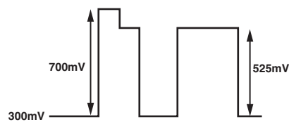
Figure 97. SD RGB Output Levels—RGB Sync Disabled
