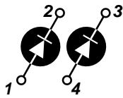
Parallel APT2X61D20J
