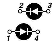
Anti-Parallel APT2X60DQ60J
