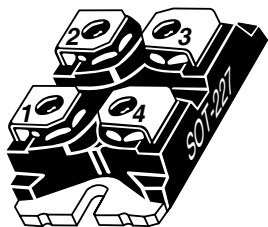
Parallel APT2X61DQ60J
