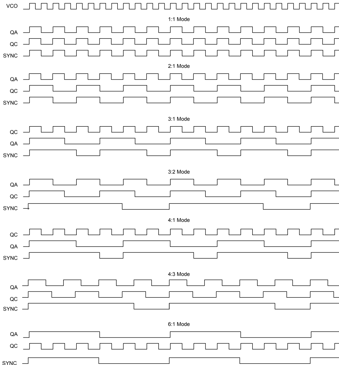
Figure 2. Timing Diagram
