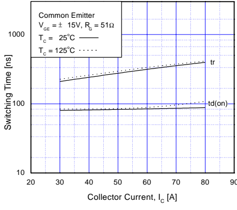
Fig 10. Turn on Characteristics vs. Collector Current
