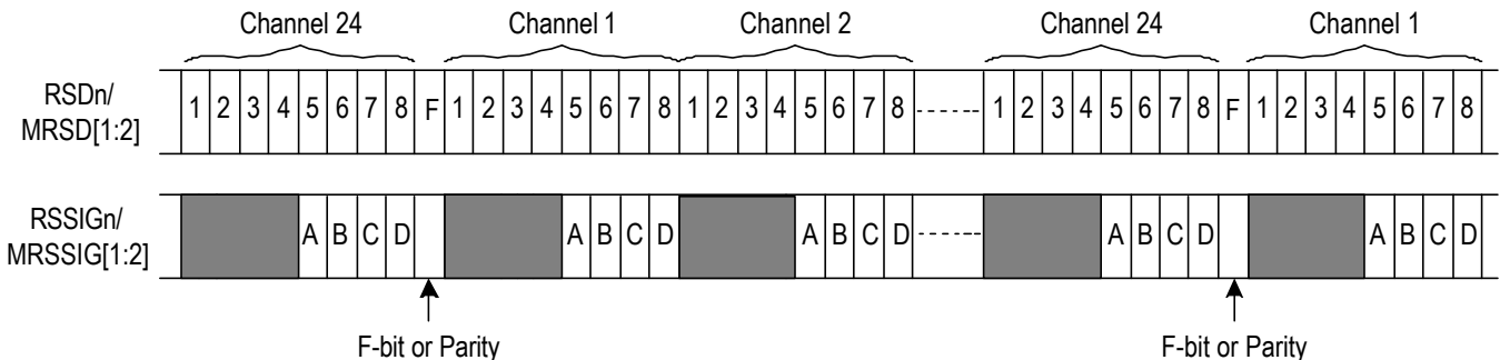
Figure - 6. Signaling Output in T1 / J1 Mode
