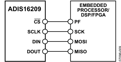
Figure 20. Typical SPI Hook-Up
