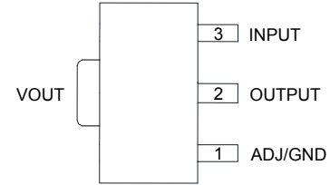
(SOT89-3L Option 2/ R Package)
