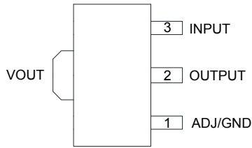
(SOT89-3L Option 1/ R Package)
