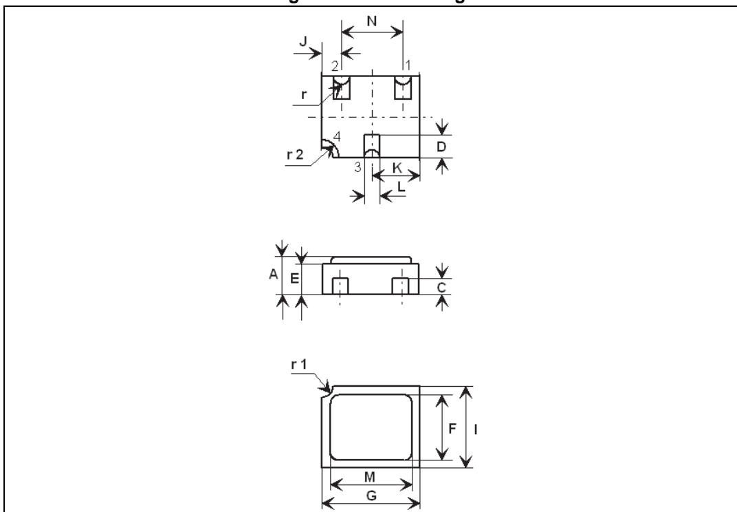
Figure 10. UB drawings
