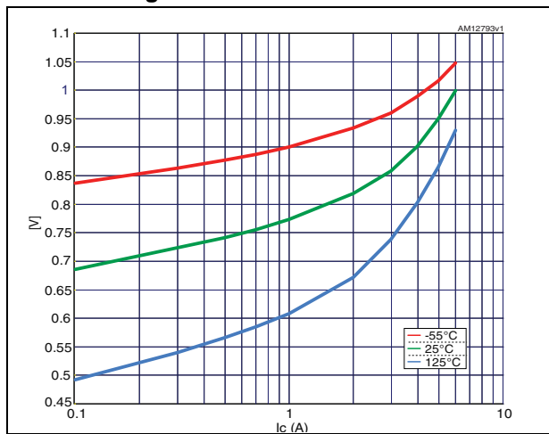
Figure 6. VBEON @ VCE = 5 V
