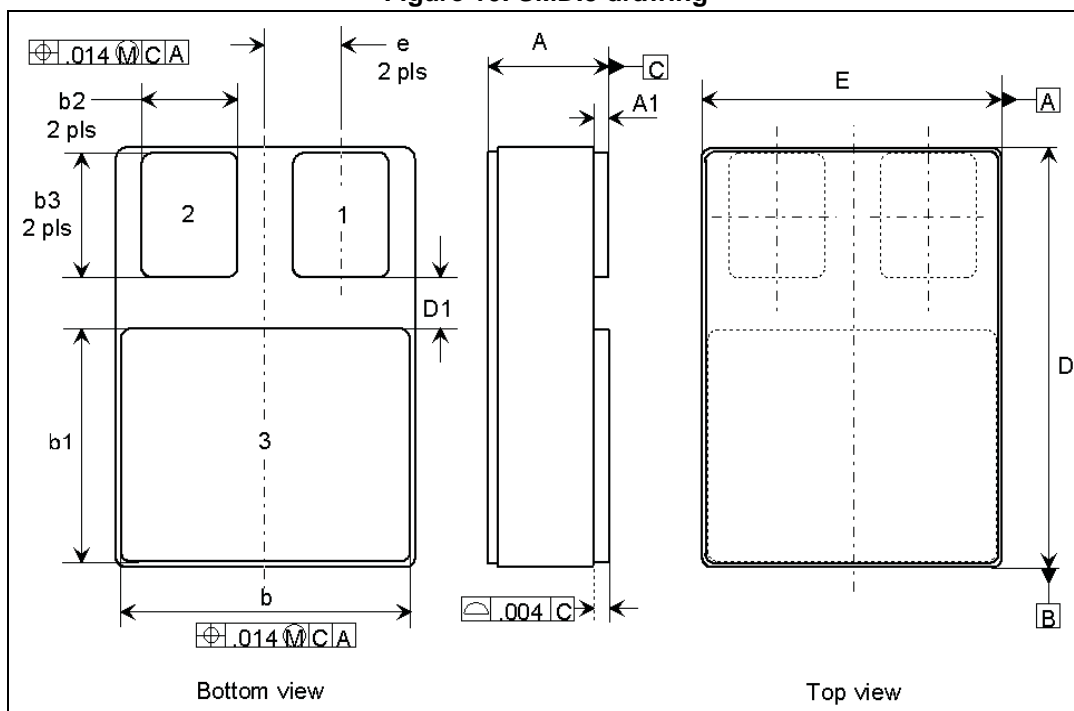
Figure 10. SMD.5 drawing
