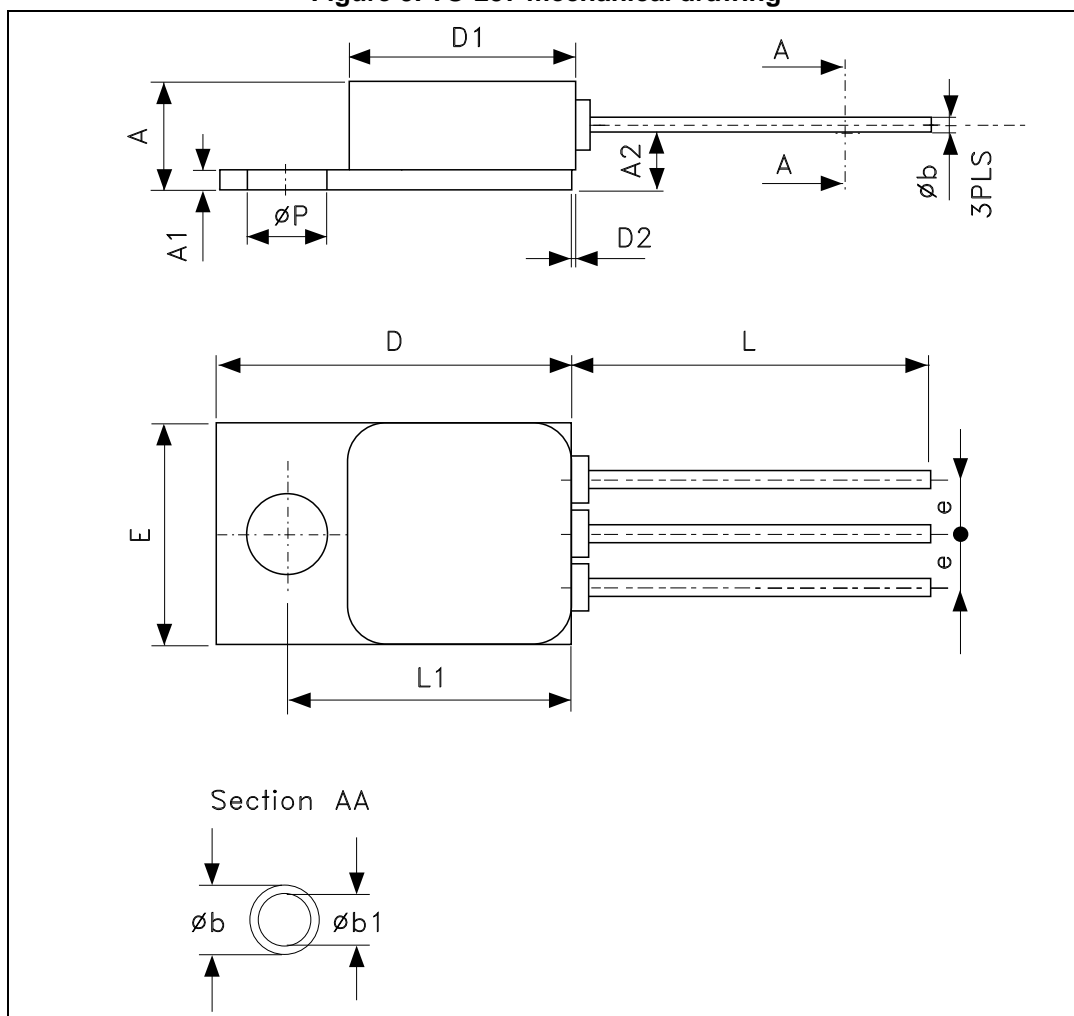
Figure 9. TO-257 mechanical drawing
