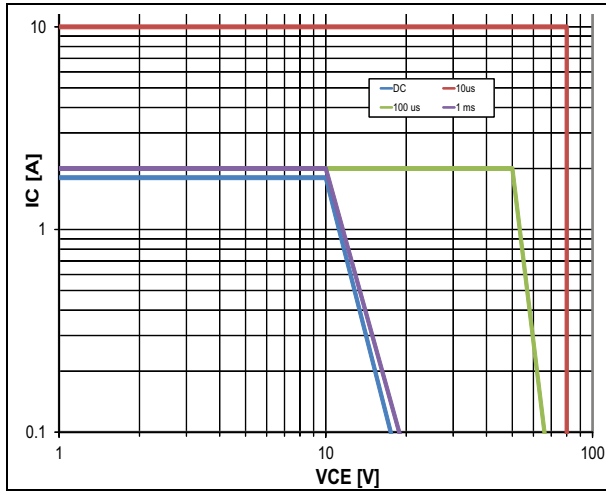
Figure 2. Safe operating area
