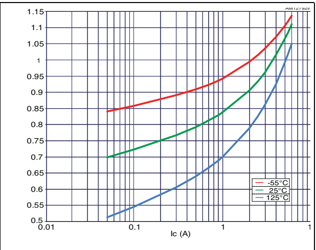
Figure 5. V_{BEsat} @ h_{FE} = 10
