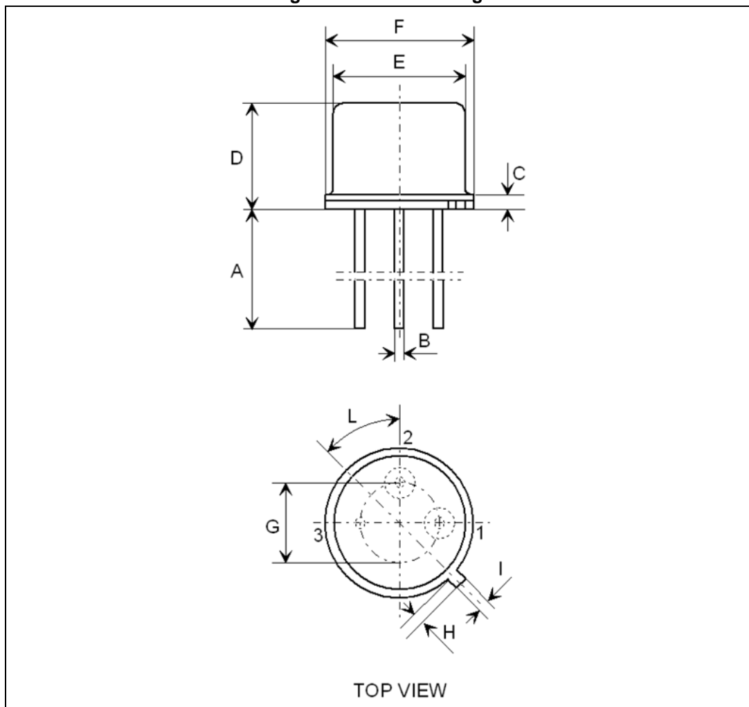
Figure 8. TO-39 drawing
