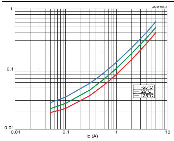
Figure 4. V_{CEsat} @ h_{FE} = 10
