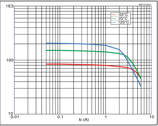
Figure 3. h_{FE} @ V_{CE} = 5
