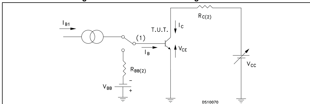
Figure 7. Resistive load switching test circuit
