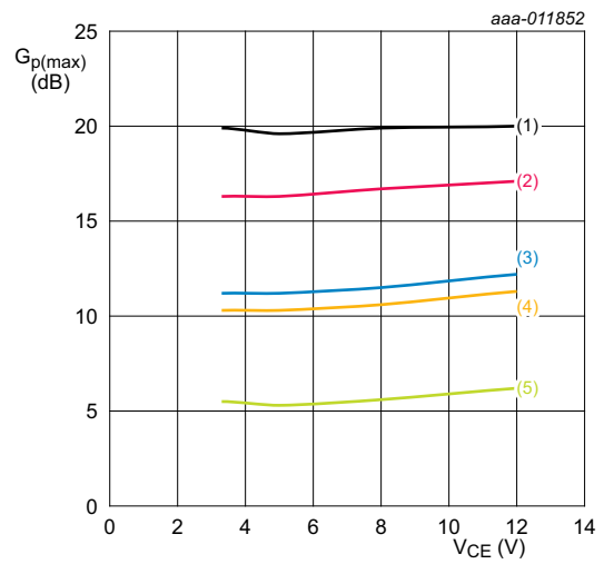
I_C = 80 mA; T_{amb} = 25 °C. If K > 1 then G_{p(max)} = maximum power gain. If K < 1 then G_{p(max)} = MSG. (1) f = 300 MHz (2) f = 433 MHz (3) f = 800 MHz (4) f = 900 MHz (5) f = 1800 MHz
