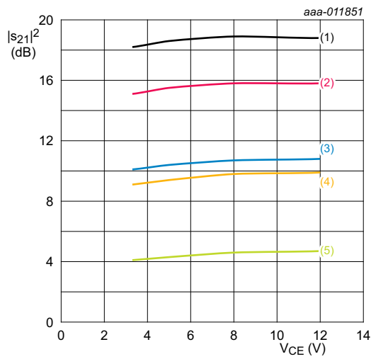
I_C = 50 mA; T_{amb} = 25 °C. (1) f = 300 MHz (2) f = 433 MHz (3) f = 800 MHz (4) f = 900 MHz (5) f = 1800 MHz
