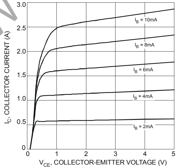
Fig. 2 Typical Collector Current vs. Collector-Emmitter Voltage
