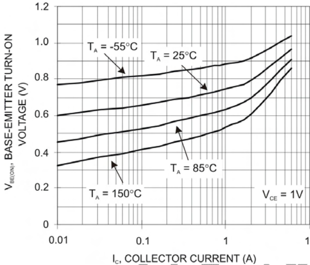
Fig. 5 Base-Emitter Turn-On Voltage vs. Collector Current
