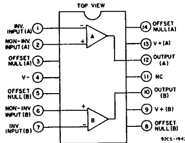
1f.—CA747CE and CA747E with internal phase compensation.
