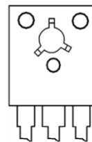
B C E Front Face View Pin-Out
