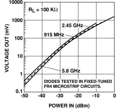
Figure 3. +25°C Output Voltage vs. Input Power, 3 μA Bias.
