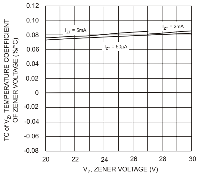
Fig. 18 Typical Temperature Coefficient of Zener Voltage, DDZX9707W - DDZX9713W
