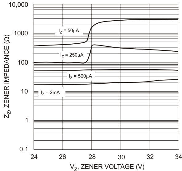
Fig. 14 Typical Zener Impedance Characteristics, DDZX9709W - DDZX9714W
