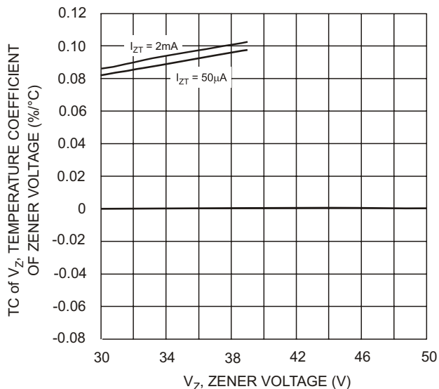
Fig. 19 Typical Temperature Coefficient of Zener Voltage, DDZ9713W - DDZ9716W
