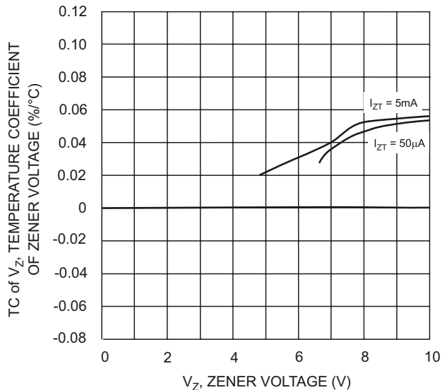
Fig. 16 Typical Temperature Coefficient of Zener Voltage vs. Zener Voltage, DDZX9692W - DDZX9697W
