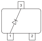
BAT68
